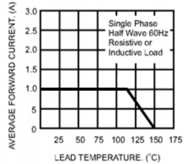
FIG.2- MAXIMUM FORWARD CURRENT DERATING CURVE
