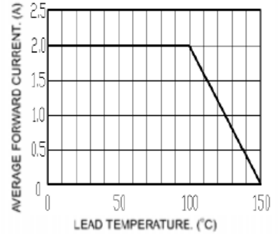
FIG.2- MAXIMUM FORWARD CURRENT DERATING CURVE
