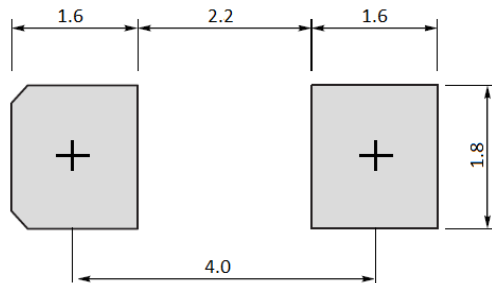
Fig.7 Mounting Pad Layout
