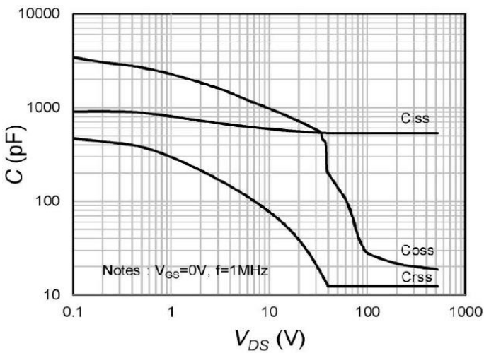
Fig.9 Capacitances
