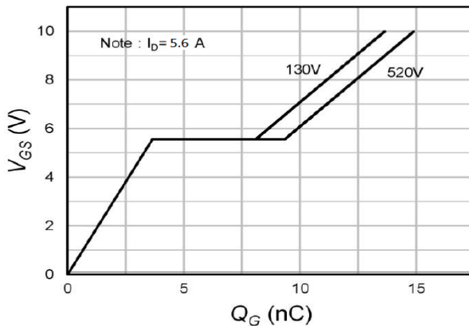
Fig.4 Gate-Charge Characteristics
