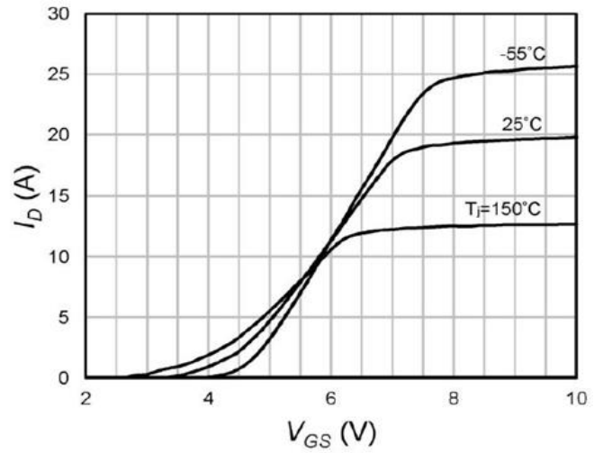
Fig.8 Transfer Characteristics
