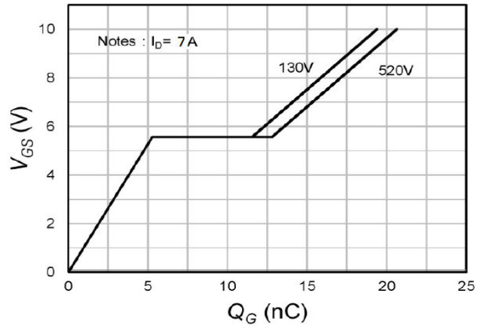
Fig.4 Gate-Charge Characteristics
