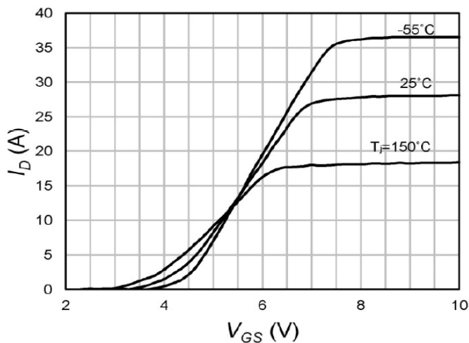
Fig.8 Transfer Characteristics
