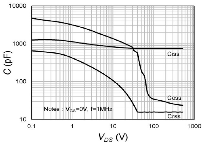
Fig.9 Capacitances
