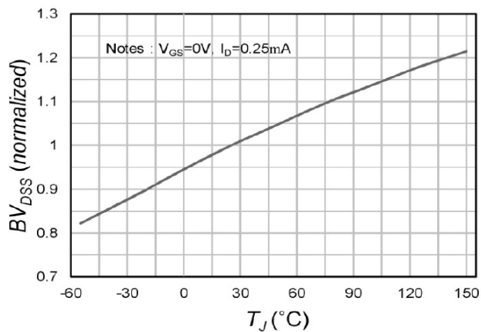
Fig.7 Drain-Source Breakdown Voltage(Normized)
