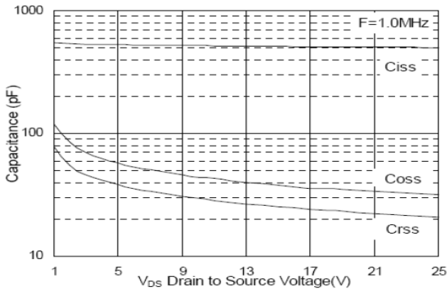
Fig.7 Capacitance
