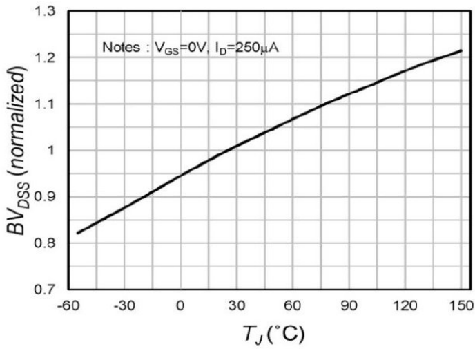
Fig.7 Drain-Source Breakdown Voltage(Normazied)
