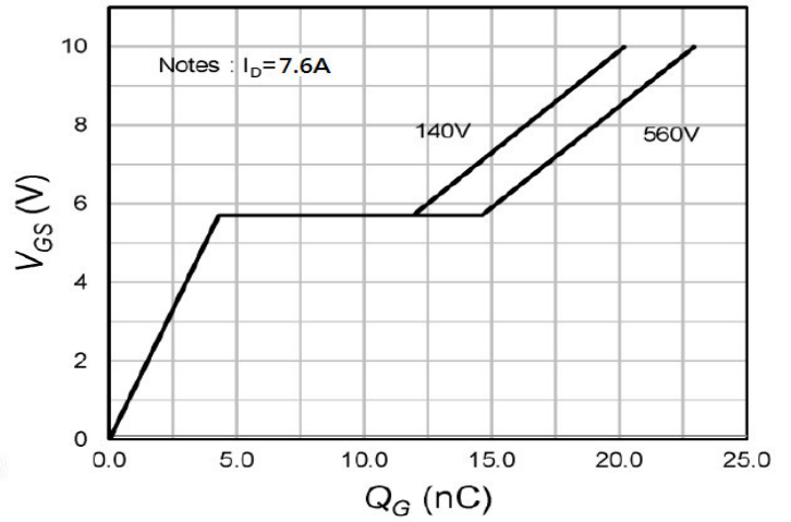
Fig.4 Gate-Charge Characteristics
