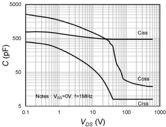
Fig.9 Capacitances
