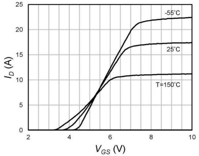
Fig.8 Transfer Characteristics
