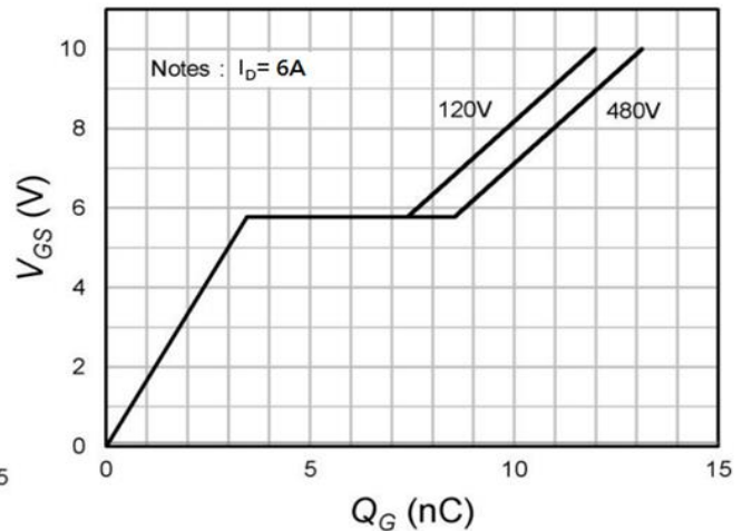
Fig.4 Gate-Charge Characteristics
