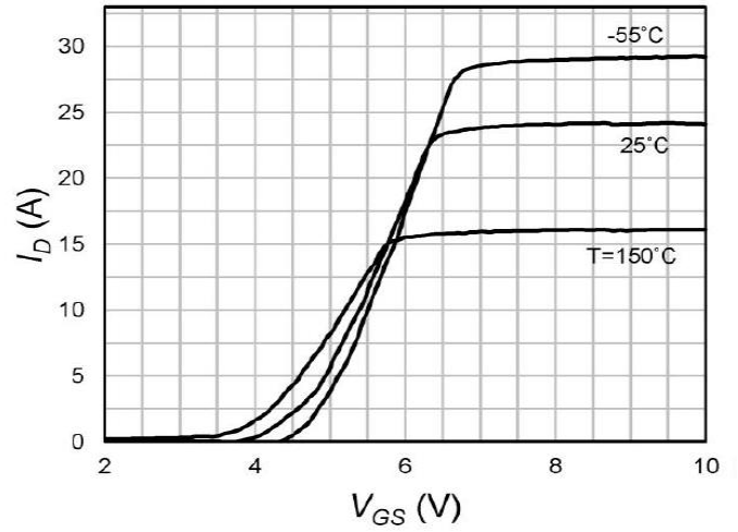
Fig.8 Transfer Characteristics
