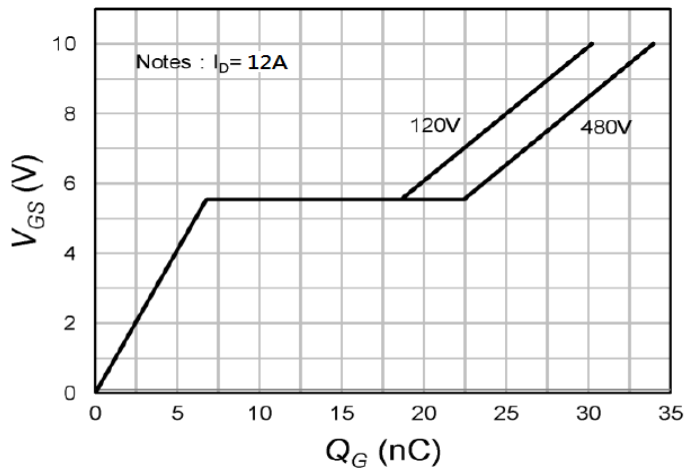
Fig.4 Gate-Charge Characteristics
