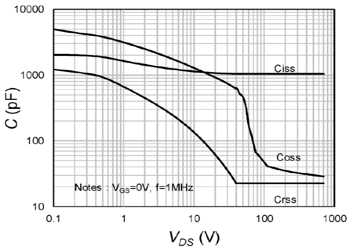
Fig.9 Capacitances
