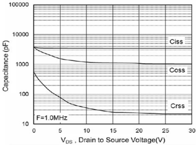
Fig.7 Capacitance
