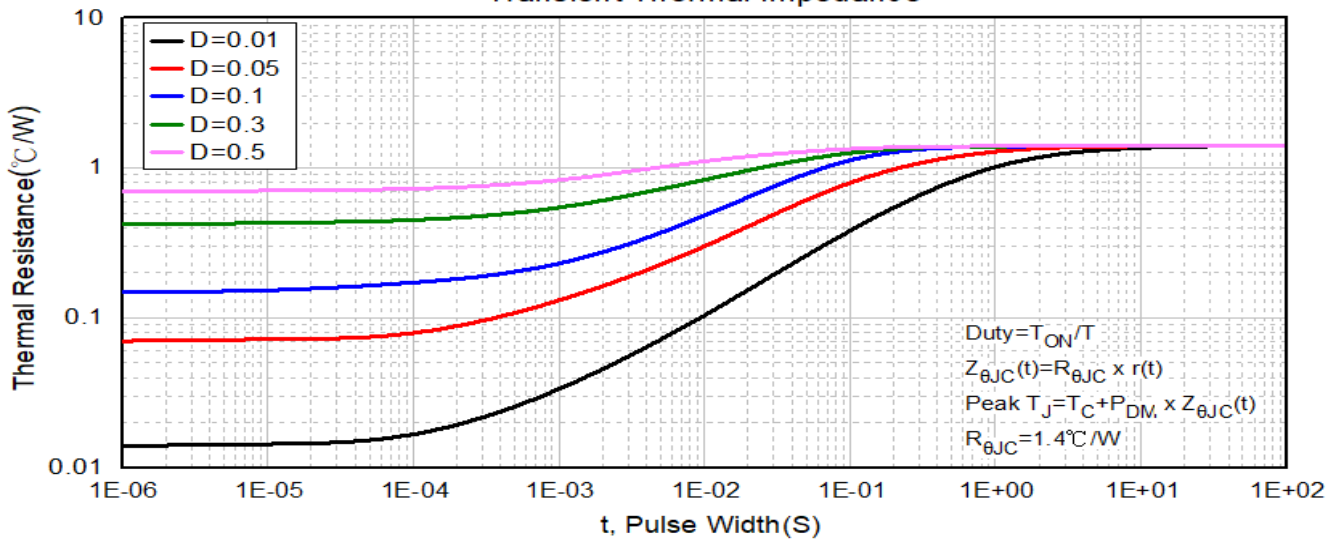
Transient Thermal Impedance
