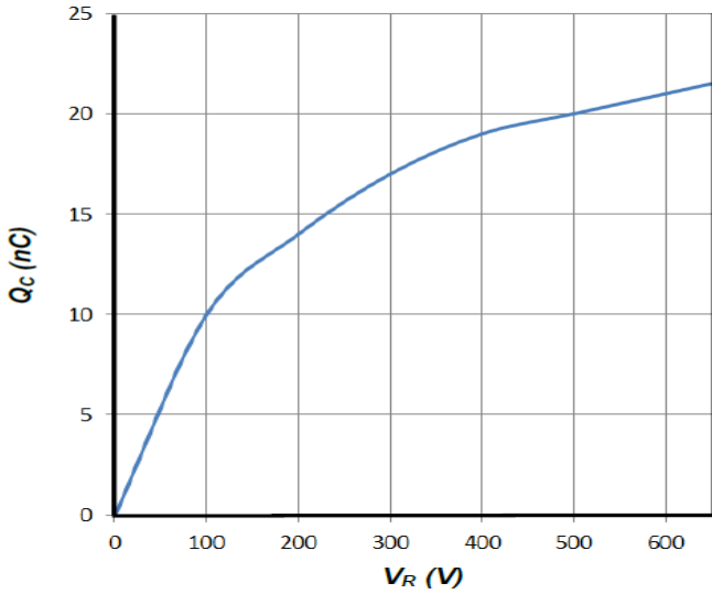
Total Capacitive Charge vs. Reverse Voltage
