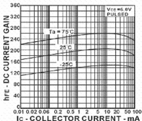
DC CURRNT GAIN vs. COLLECTOR CURRENT
