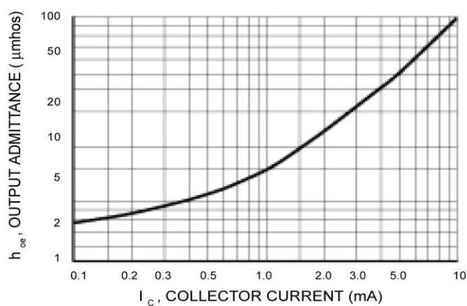
Figure 10. Output Admittance
