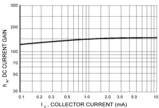
Figure 9. Current Gain
