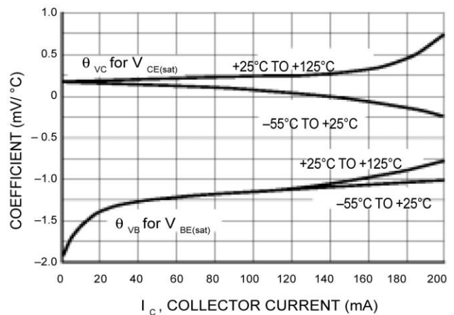
Figure 16. Temperature Coefficients
