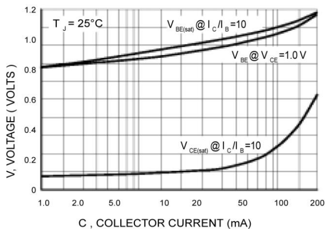
Figure 15. "ON" Voltages
