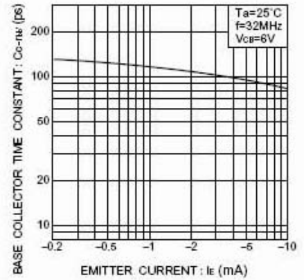
Fig.12 Base-collector time constant vs. emitter current
