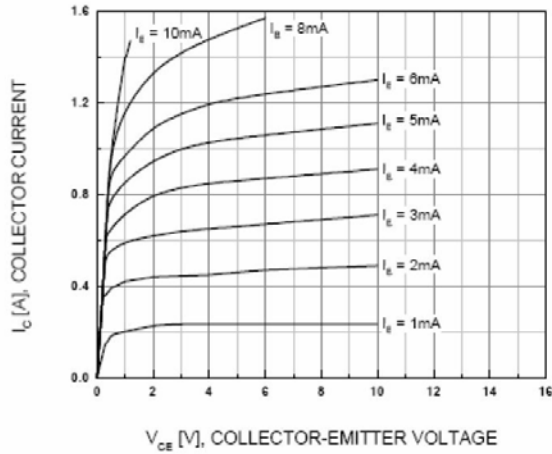
Figure 1. Static Characteristics
