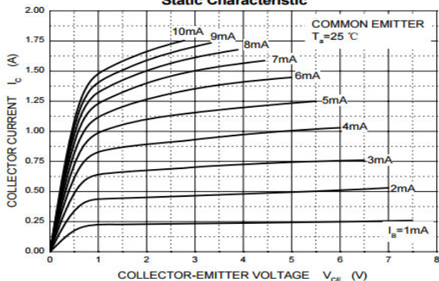
Static Characteristic
