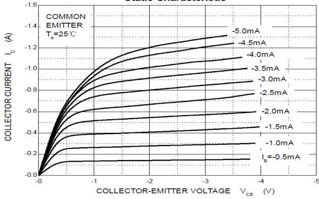
Static Characteristic
