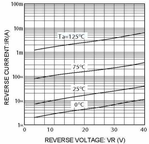
Fig.2 Reverse characteristics
