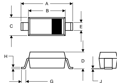
SOD-123
