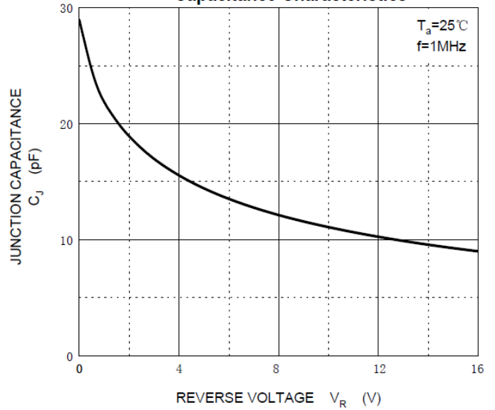
Capacitance Characteristics
