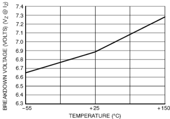
Figure 1. Typical Breakdown Voltage versus Temperature
