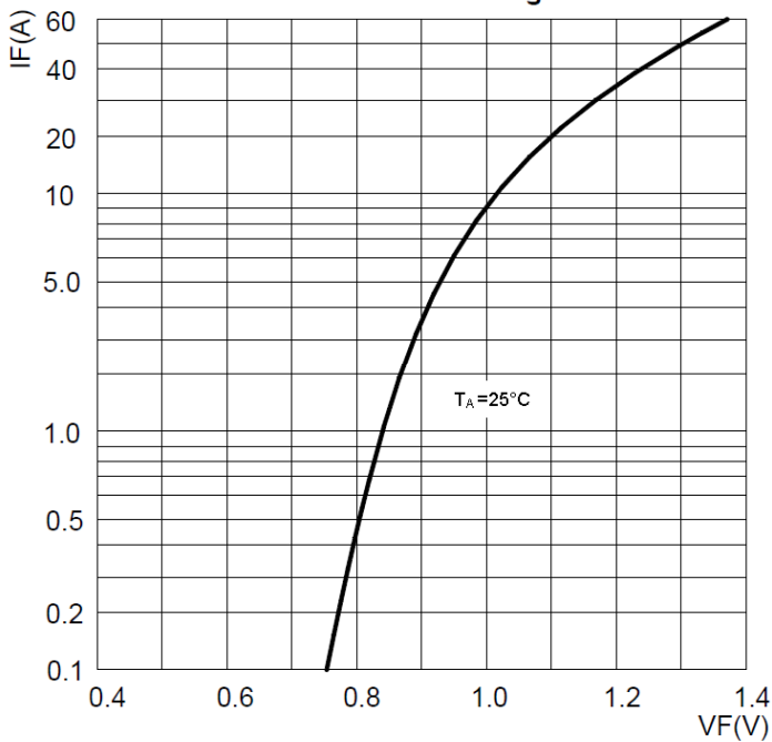
FIG3: Forward Voltage
