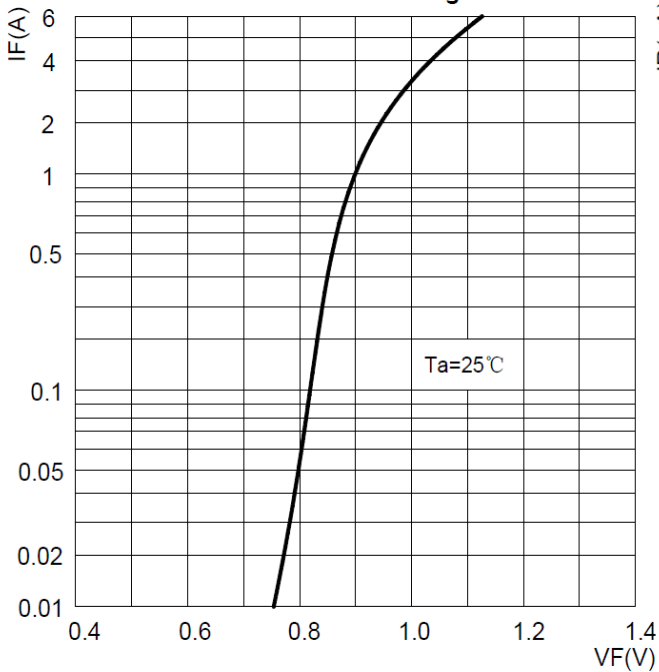
FIG3: Forward Voltage
