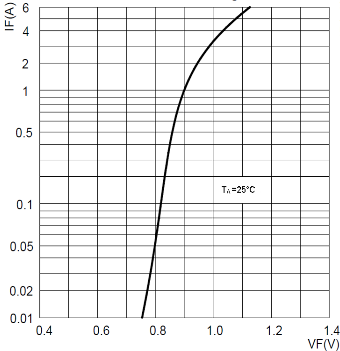
FIG3: Forward Voltage
